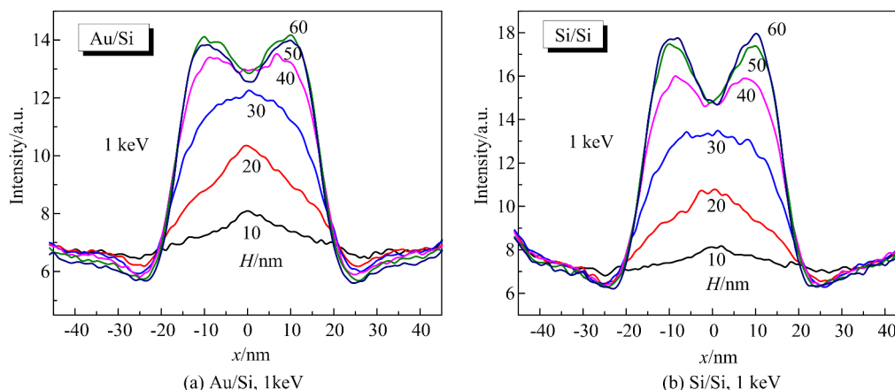
Fig.3 Simulated SE line-scans of a wave-type line structure on a substrate at different heights for the bottom width of W=50 nm and \alpha_1=\alpha_2=100
